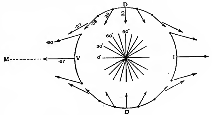
FIG. 2.—Tide-generating Force.
