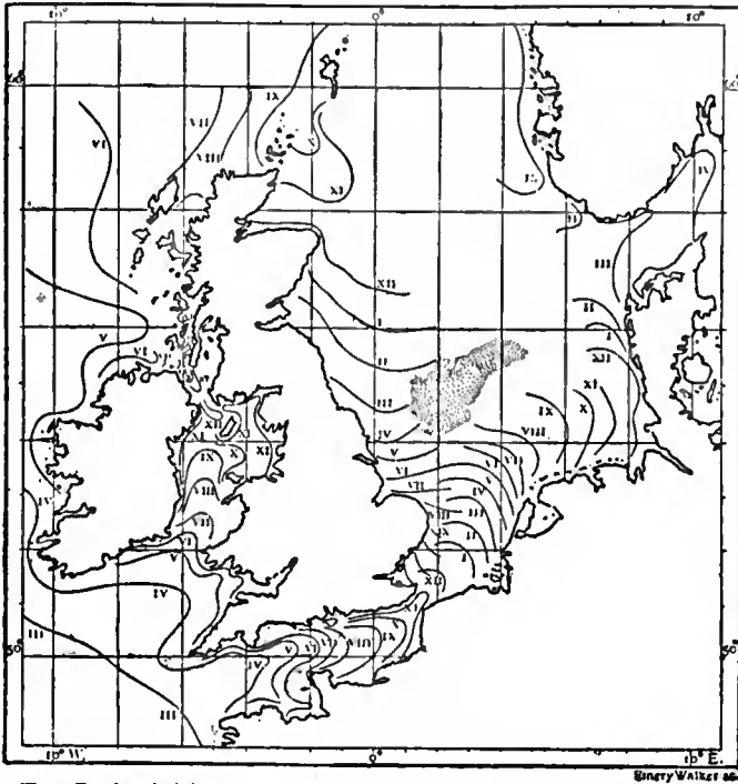
FIG. 3.—Cotidal Lines in British Seas.
