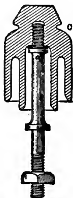
FIG. 2.—Cordeaux Insulator.
