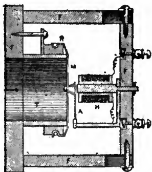
FIG. 1.—Bell's First Telephone (1875); one-fifth full size.
