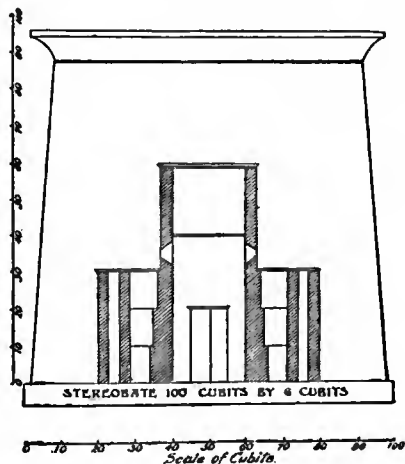
FIG. 4.—Diagrammatic Section of Herod's Temple and Porch.
