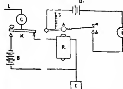
FIG. 18.—Single-current Relay Working.
