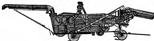
FIG. 4.—American "Separator" with self-feeder and fan-blast delivery-pipe for straw. (Avery Manufacturing Co., Peoria, Illinois.)
