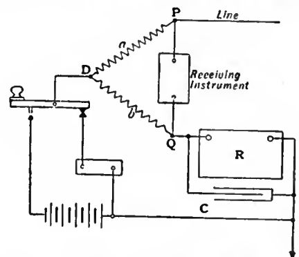
FIG. 24.—Duplex Working: bridge method.
