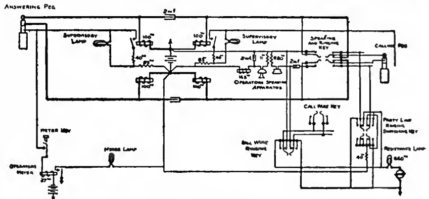
FIG. 13.—Typical Cord Circuit, British Insulated Co.'s System.
