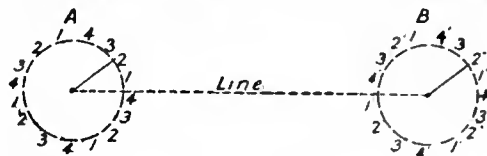
FIG. 27.—Grouping of Segments in Multiplex System.
