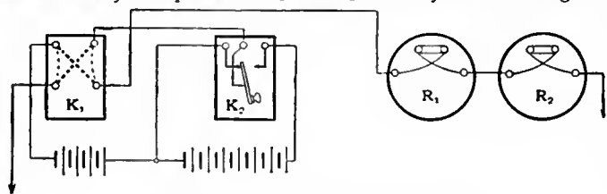
FIG. 25.—Quadruplex Working.
