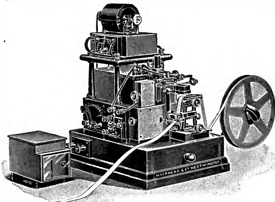
FIG. 32.—Muirhead's Siphon Recorder.
