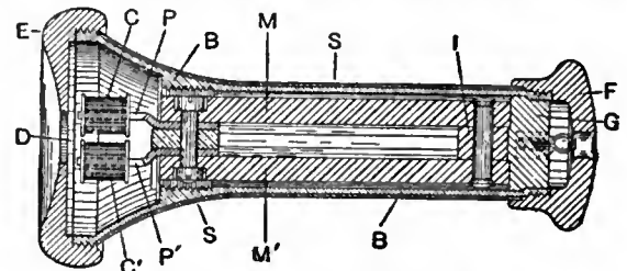
FIG. 3.—Double Pole Receiver.
