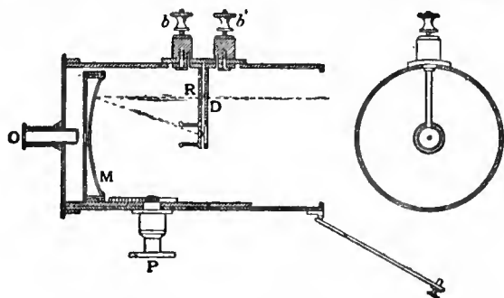
FIG. 8.—Féry's Mirror Pyrometer (Camb. Scient. Inst. Co.). For temperatures from 500^{\circ}\text{C.} to 1100^{\circ}\text{C.}
