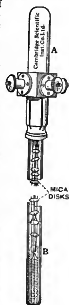
FIG. 7.— Platinum Thermometer.
