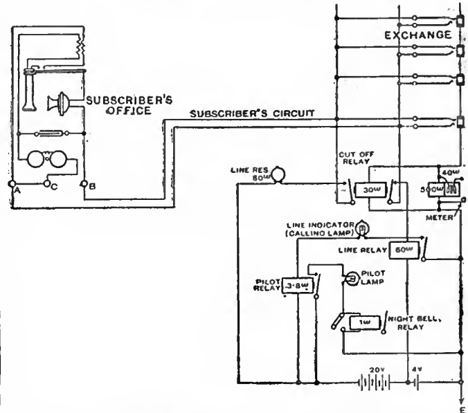
FIG. 11.—Subscriber's Circuit, Common Battery System.
