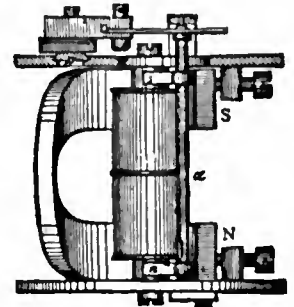
FIG. 20.—Post Office Standard Relay.
