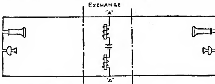
FIG. 9.—Stone Common Battery System.
