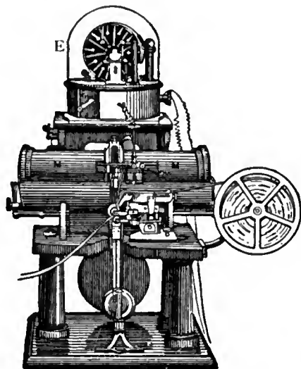
FIG. 31.—Lord Kelvin's early Siphon Recorder.
