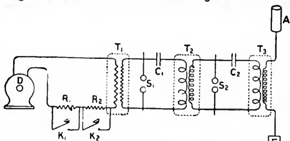
FIG. 43.—Alternate Current Transformer System. (Fleming.)
