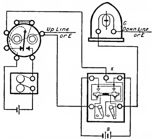
FIG. 21.—Connexions for Double-current Working.
