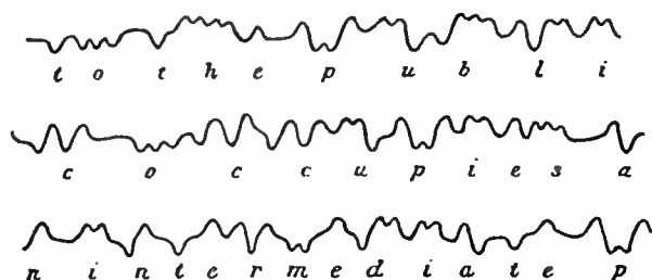
FIG. 33.—Facsimile of Siphon Recorder Message.
