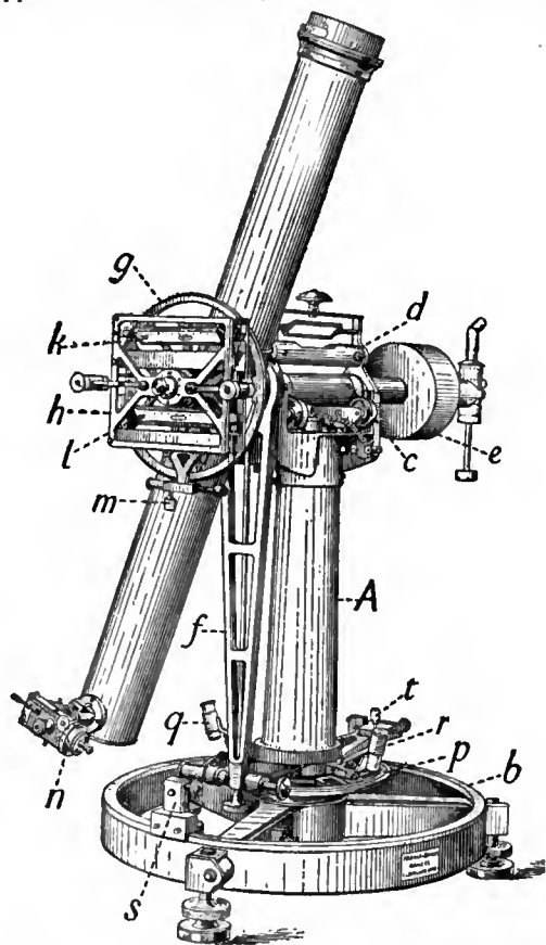
FIG. 24.—Zenith Telescope (by Warner & Swasey).
