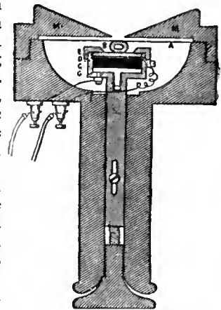
FIG. 4.—Edison's Microphone Transmitter.
