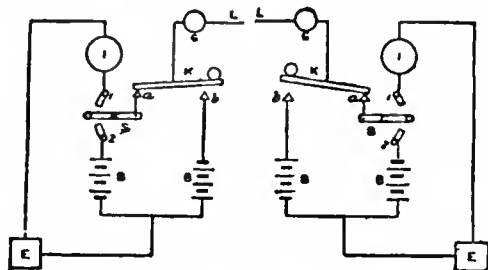
FIG. 22.—Universal Battery Working.
