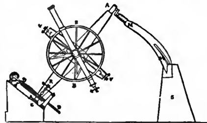
FIG. 10.—Equatorial Telescope. English form.
