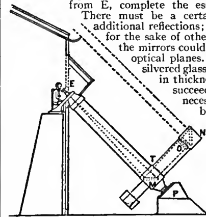
FIG. 22.—Loewy's Coudé Equatorial.
