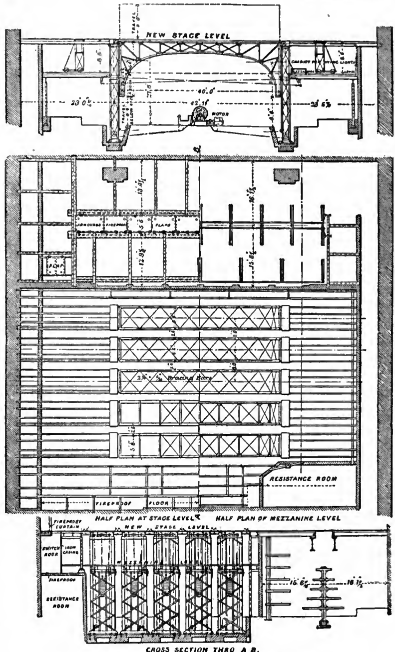
FIG. 6.—Plan and Section of Covent Garden Stage.
