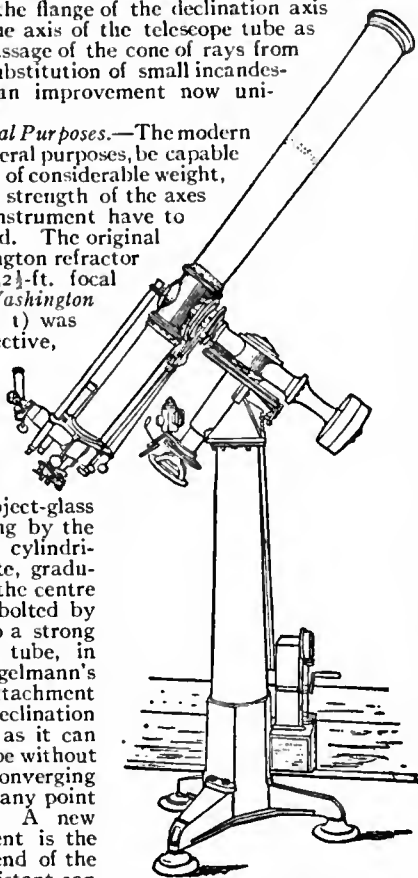
FIG. 15.—Dr Engelmann's 8-in. Refractor.
