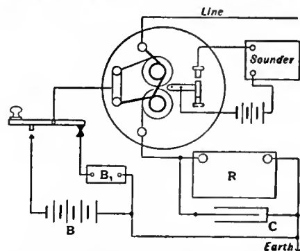
FIG. 23.—Duplex Working: differential method.
