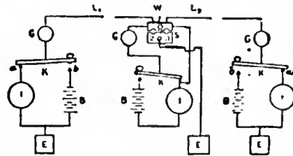
FIG. 16.—Open Circuit, Single-current System.
