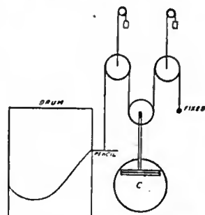
FIG. 4.—Tide-Predicting Instrument.
