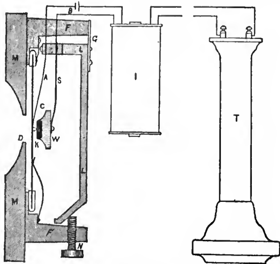
FIG. 5.—Blake's Transmitter.
