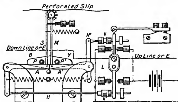
FIG. 29.—Wheatstone Automatic Transmitter.
