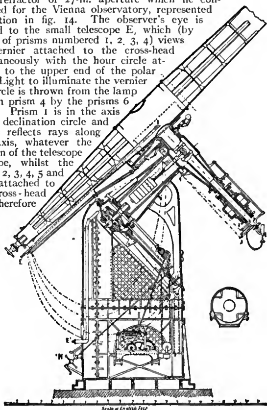
FIG. 14.—Grubb's 27-in. Refractor (Vienna).
