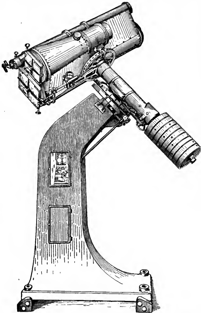
FIG. 19.—Bruce Telescope, made for the Yerkes Observatory.
