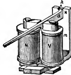
FIG. 19.—Siemens Polarized Relay.
