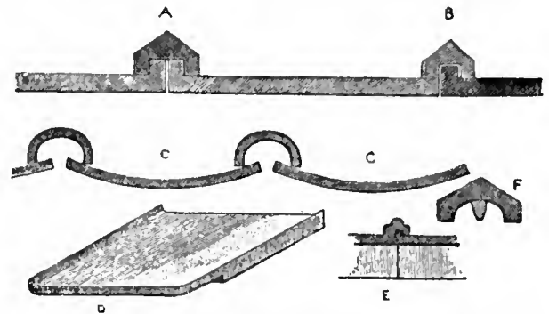
FIG. 1.—Examples of roofing tiles from Greek Temples.
