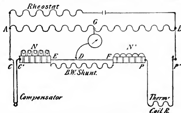
FIG. 6.—Diagram of Compensated Bridge Method.
