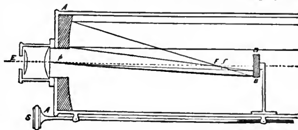
FIG. 7.—Gregorian Telescope.
