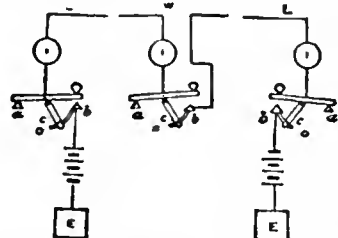
FIG. 17.—Closed Circuit, Single-current System.
