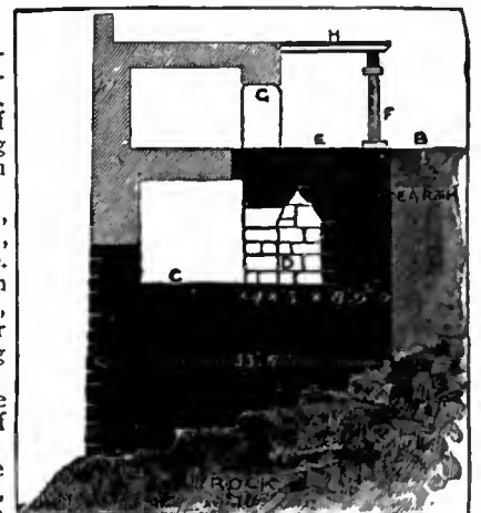
FIG. 2.—Section through the Outer Wall of the City at 20 in fig. 1.
