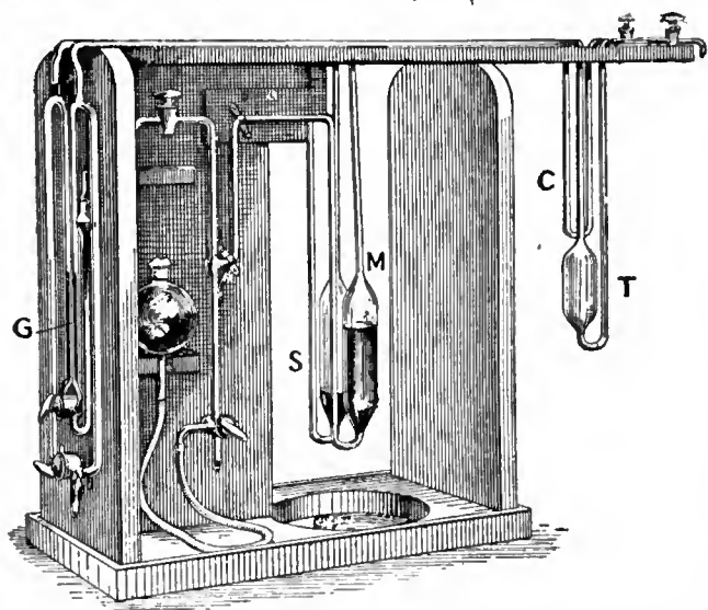
FIG. 5.—Compensated Differential Gas Thermometer.
