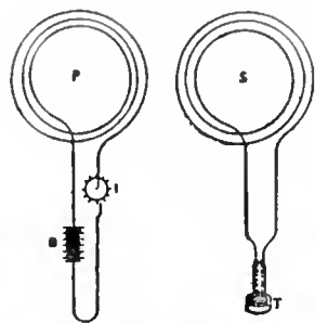
FIG. 36.—Magneto-Induction Method.
