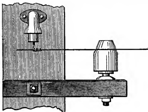
FIG. 3.—Terminal Insulator.
