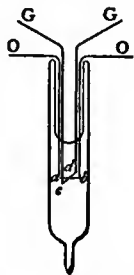
FIG. 48.—Tellurium-bismuth Vacuum Thermal Detector for Electric Oscillations. a b , constantan wire; c d , thermojunction; G G , galvanometer terminals; O O , antenna and earth terminals.
