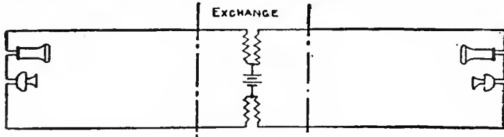
FIG. 8.—Hayes Common Battery System.
