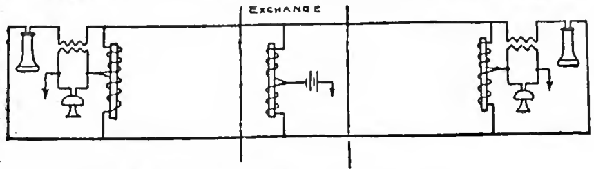
FIG. 10.—Dean Common Battery System.
