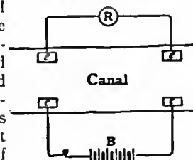
FIG. 35.—Morse's Conduction Method.
