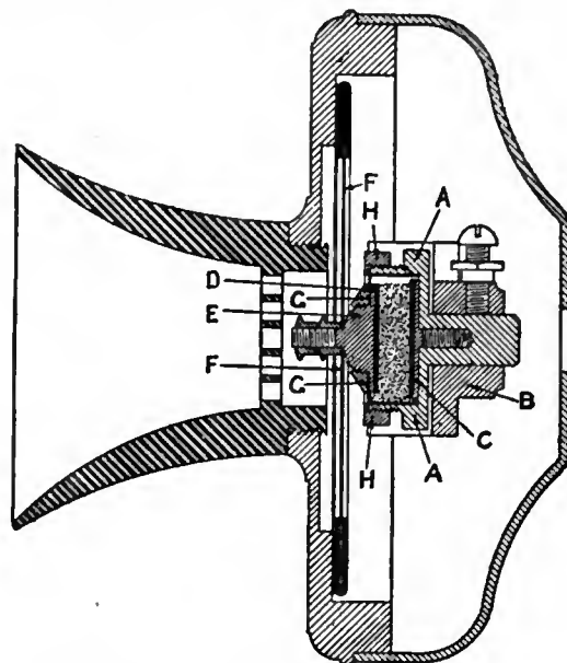
FIG. 6.—Solid Back Transmitter.
