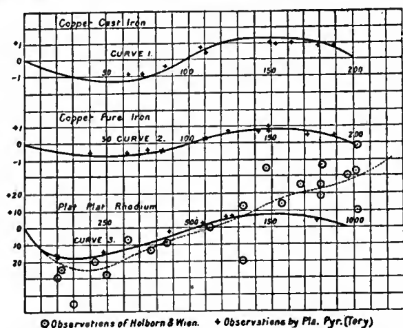
FIG. 2.—Temperature by Thermocouple. Difference from Tait's Formula.
